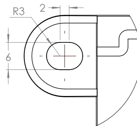
DETAIL A 2x SCALE 2:1
